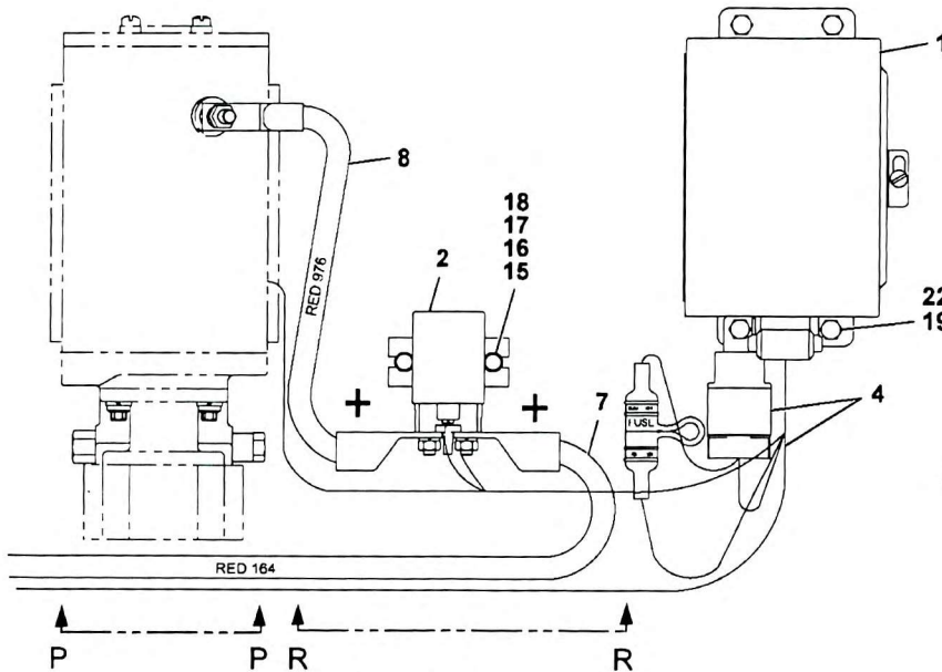
DETAIL B EMERGENCY STEER PUMP RELAY AND BOX ROTATED 90° CW
